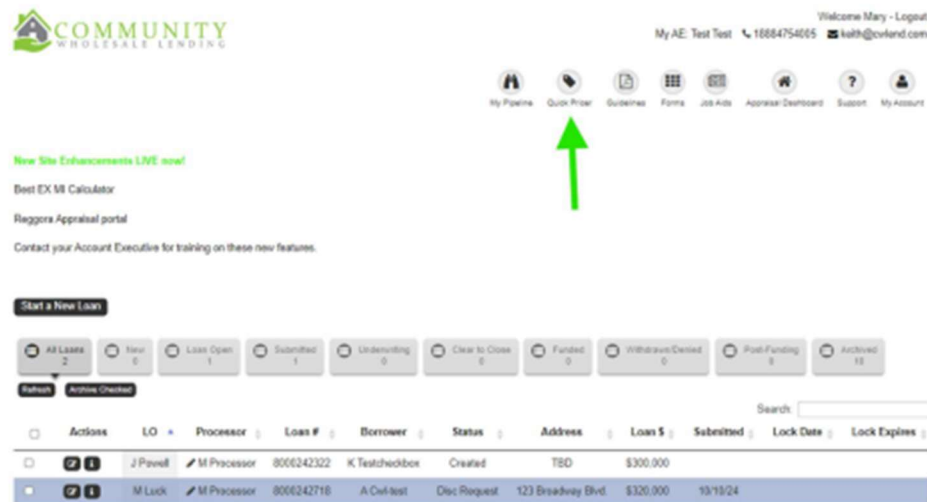
Figure 2. Quick Pricer
