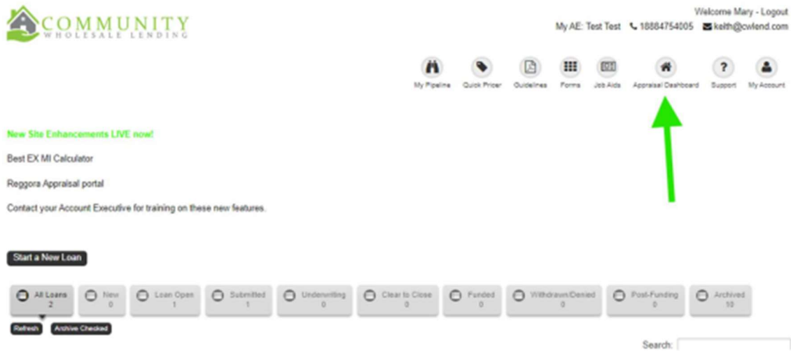
Figure 6. Appraisal Dashboard
